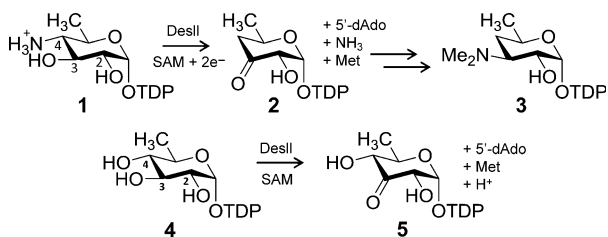
Scheme 1. Reactions catalyzed by DesII.
