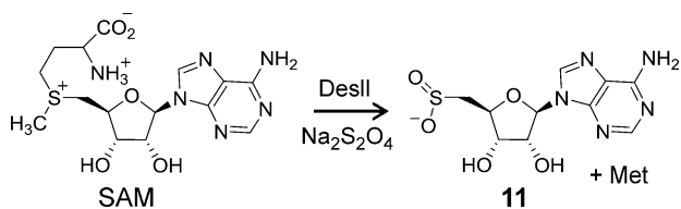
Scheme 2. Conversion of SAM to 11 in the presence of DesII and Na 2 S 2 O 4
